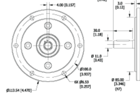
Flange Option 5
