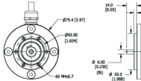
Flange Option 5
