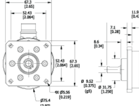
Flange Option 4
