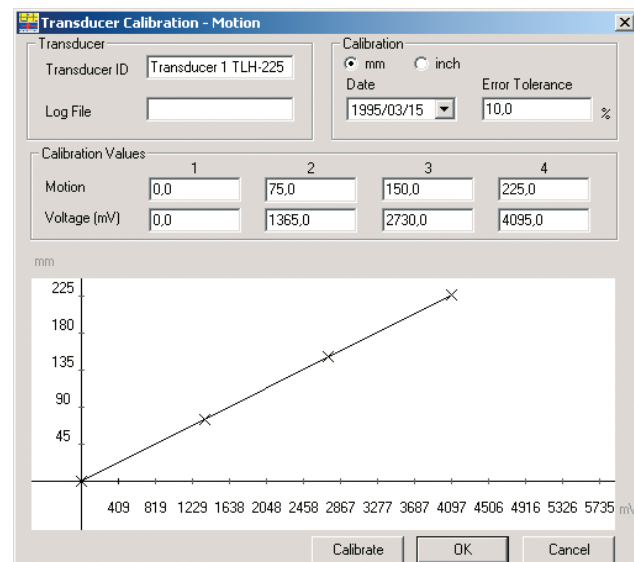
Figure 2. Linear and angular travel, voltage, current, pressure and vibration transducers can be defined and calibrated with CABA Win
